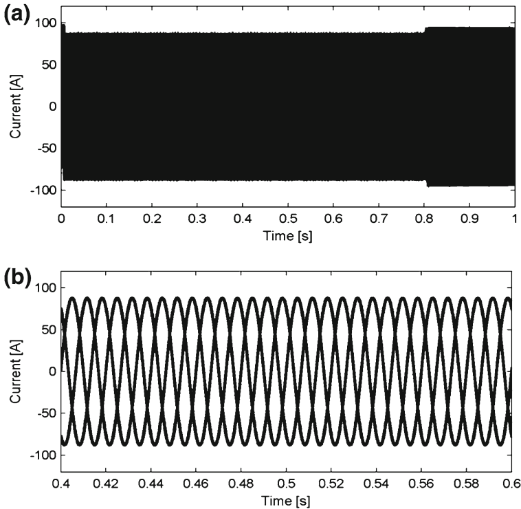
Fig. 17 a Load current waveforms and b zoom of (a)
